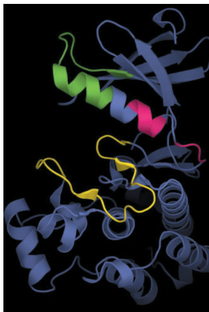
Figure 1 Similar positioning within the epidermal growth-factor receptor (EGFR) kinase domain (database accession numbers MMD8:20494/PDB:1M17) of the EGFR and ERBB2 mutations that are found in a proportion of lung tumours. The composite position of reported EGFR deletions 2,3 is indicated in green; the relative positions of the ERBB2 insertions described here are mapped onto the EGFR sequence and are shown in pink. The first third of the activation loop of the kinase domain is indicated in yellow for orientation.
